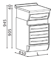
CM4/ET50 L.520
